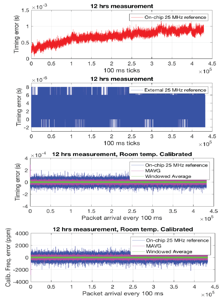
Fig. 8 Timing accuracy for the 100 ms time interval. The top plot shows the timing error due to the free-running 25 MHz reference. The second plot from the top shows the timing error due to an external 25 MHz crystal frequency reference. The third & fourth plot from the top shows the measured calibrated timing and frequency error respectively.
