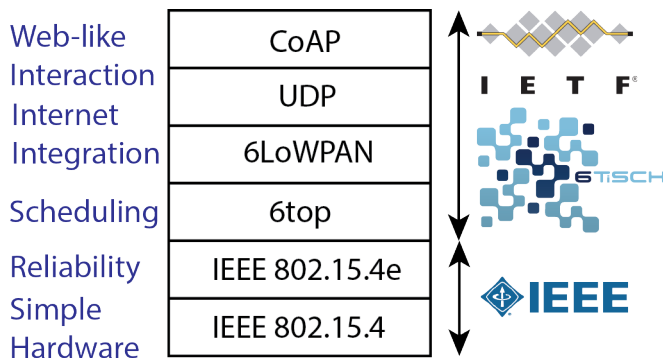
Fig. 15 Network stack
