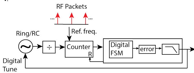
Fig. 4 Network referenced FLL.
