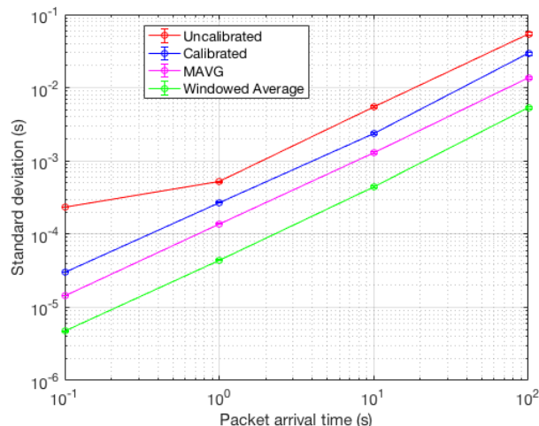
Fig. 10 Measured timing error as a function of packet arrival time.
