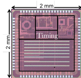
Fig. 5 Die photo of the test chip in 65 nm CMOS.
