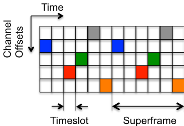
Fig. 14 An example communication schedule.
