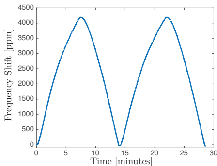
Fig. 8. Frequency deviation during two 0^\circ\text{C} to 50^\circ\text{C} temperature ramps at 7^\circ\text{C}/\text{min} rate.
