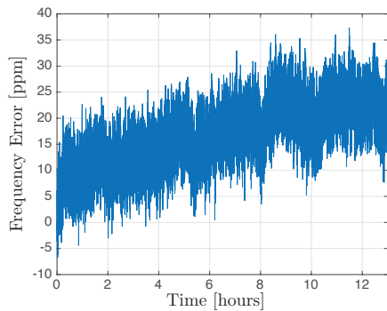
Fig. 7. Measured LO stability at bias current of 500 \mu\text{A} .
