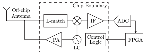
Fig. 1. System level block diagram of the transceiver.
