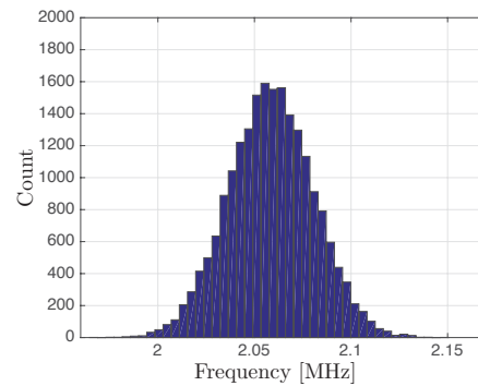
Fig. 6. Histogram ( \sigma = 22\text{kHz} ) of instantaneous IF frequency down-converted by free-running LC tank over 10 ms time span.
