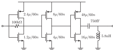
Fig. 10. Class D PA schematic.
