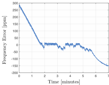
Fig. 9. Intermediate frequency of a receiver using feedback based on packets received from a transmitter whose temperature varies at 2^{\circ}\text{C}/\text{min} .
