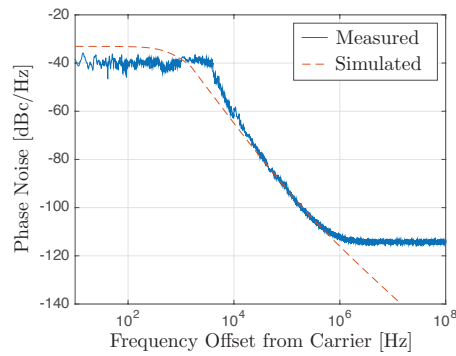
Fig. 5. LC tank phase noise measurement.
