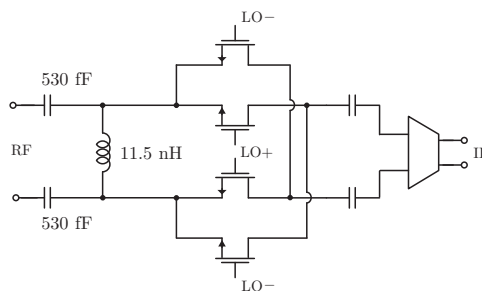
Fig. 3. Receiver front end schematic. Not pictured are off-chip RF balun and baseband filters.
